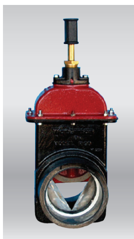
H-30 with V-notch opening
